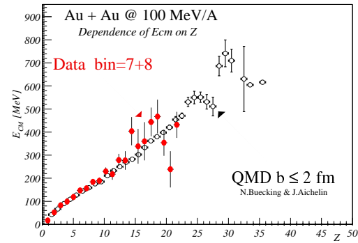
FIGURE 6. Comparison of the experimental mean kinetic energy as a function of the charge of the fragment obtained for central collisions (bins 7 and 8, see text) with the predictions of the QMD code.
