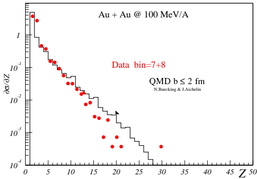
FIGURE 5. Comparison of the experimental fragment size distributions obtained for central collisions (bins 7 and 8, see text) with the predictions of the QMD code.
