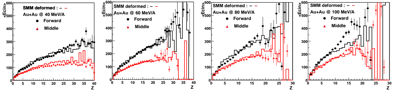
FIGURE 4. Comparison of the kinetic energy distributions (bin 7 and 8, see text) as a function of the charge of the detected ions obtained at various incident energies and for two angular ranges (forward: 0^\circ \leq \theta_{cm} \leq 60^\circ , middle: 60^\circ \leq \theta_{cm} \leq 120^\circ ). The histograms give the predictions of the statistical model SMM with an ellipsoidal freeze-out volume and a self-similar radial flow. Parameters used in the calculations are given in table 1.
